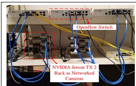
Fig. 2 Networked Camera System.
